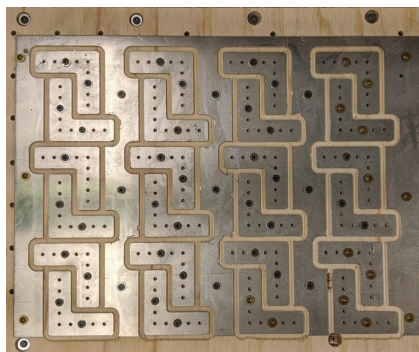
Gussets machined on the router
